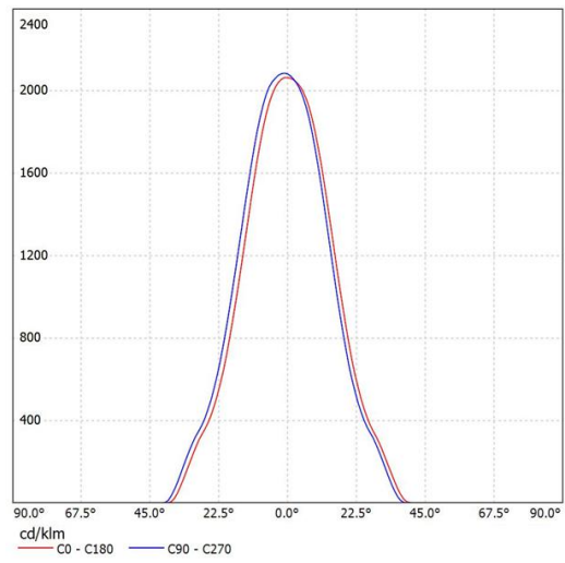
SL-05038A K:2.64cd/lm,LED:1507
