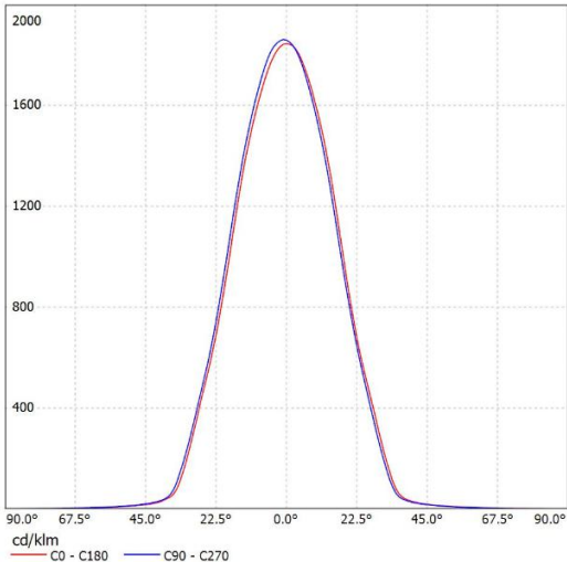
SL-05038A K:2.20cd/lm,LED:CLL02X
