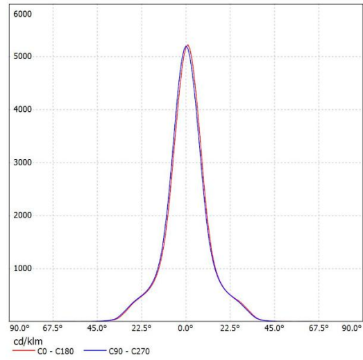
SL-05015A K:6.06cd/lm,LED:CLL02X
