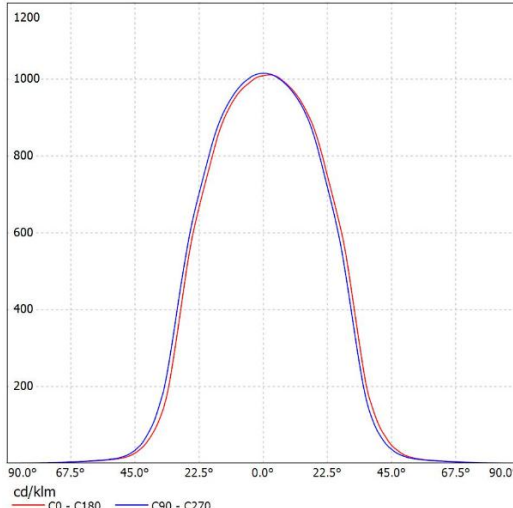
SL-05060A K:1.26cd/lm,LED:CLL02X
