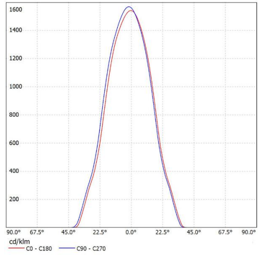
SL-05038A K:2.26cd/lm,LED:CXM-9
