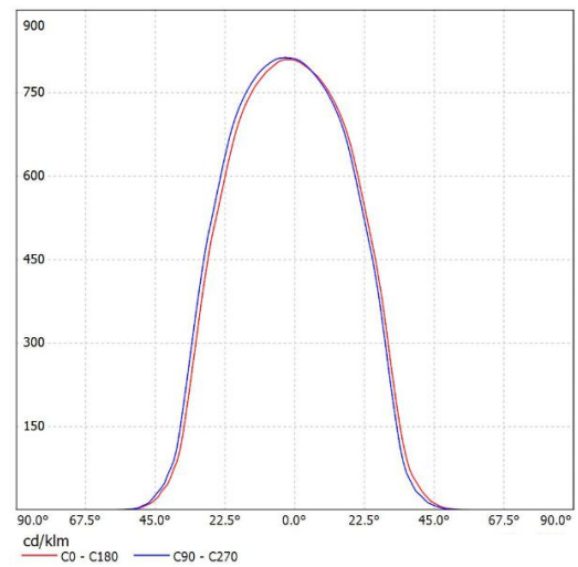
SL-05060A K:1.31cd/lm,LED:CXM-9
