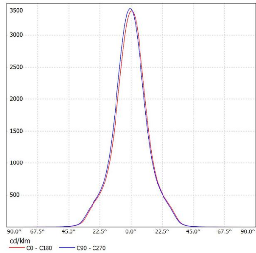
SL-05024A K:3.99cd/lm,LED:CLL02X
