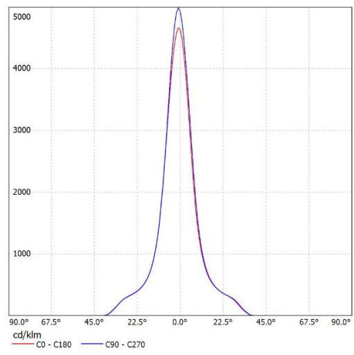
SL-05015A K:7.26cd/lm,LED:CXM-9
